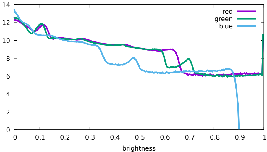
Flat histogram - Canon, EOS 5D Mark IV, 3200 ISO (7M9A0098)
