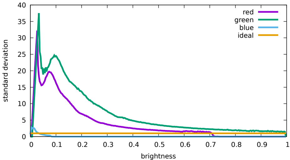
Flat noise levels - Canon, EOS 5D Mark IV, 3200 ISO (7M9A0097)
