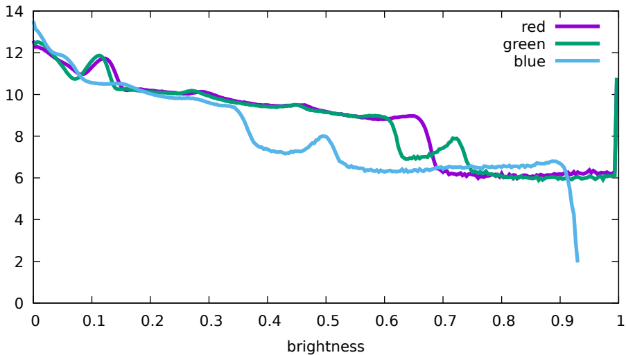
Flat histogram - Canon, EOS 5D Mark IV, 3200 ISO (7M9A0097)
