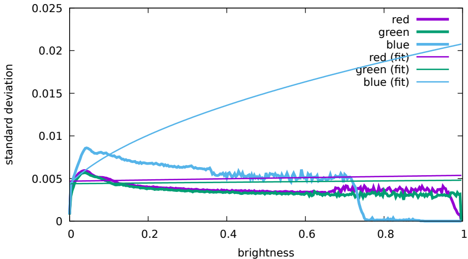
Noise levels - Canon, EOS 5D Mark IV, 3200 ISO (7M9A0098)
