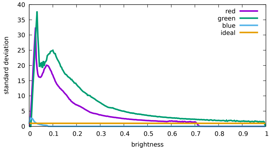
Flat noise levels - Canon, EOS 5D Mark IV, 3200 ISO (7M9A0098)
