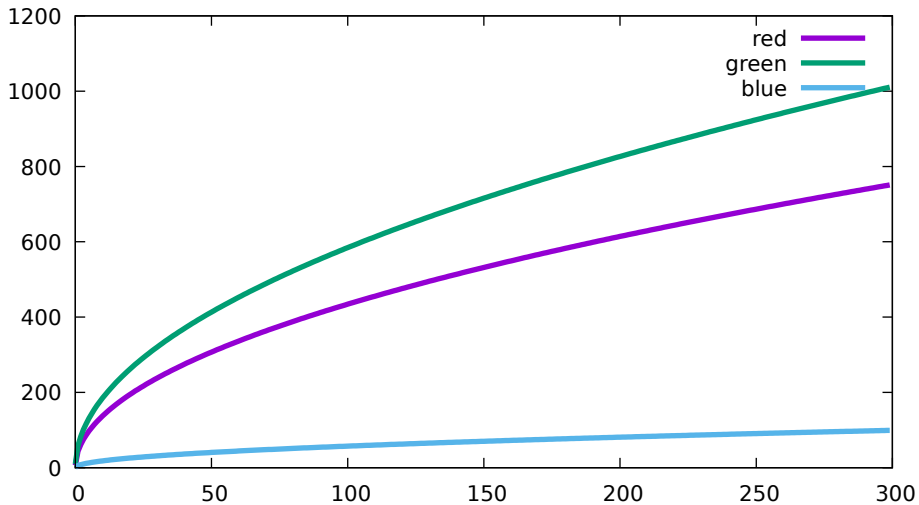
Conversion curves - Canon, EOS 5D Mark IV, 3200 ISO (7M9A0097)
