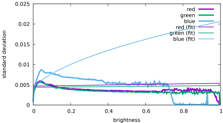
Noise levels - Canon, EOS 5D Mark IV, 3200 ISO (7M9A0097)
