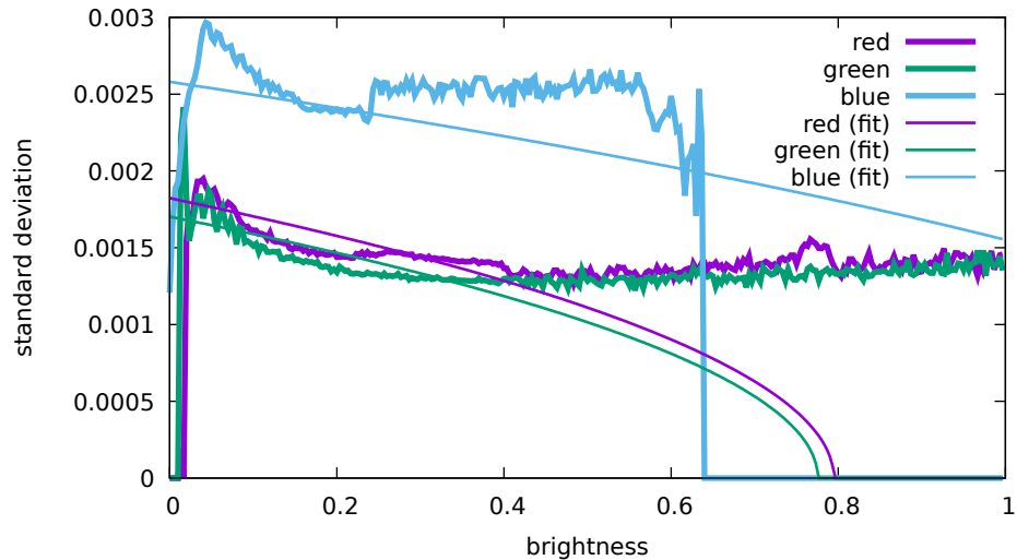
Noise levels - Canon, EOS 5D Mark IV, 400 ISO (7M9A0061)
